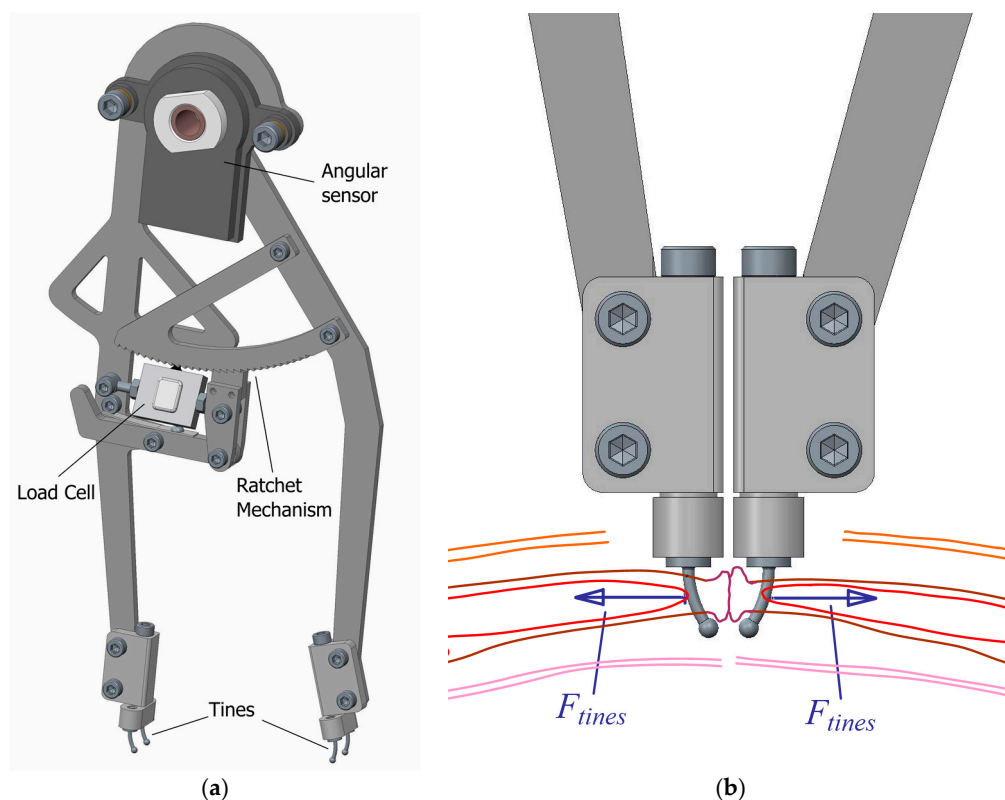
Figure 2. Instrument: (a) Conceptual design; (b) Forces applied by the aponeurotic edges to the tines.
